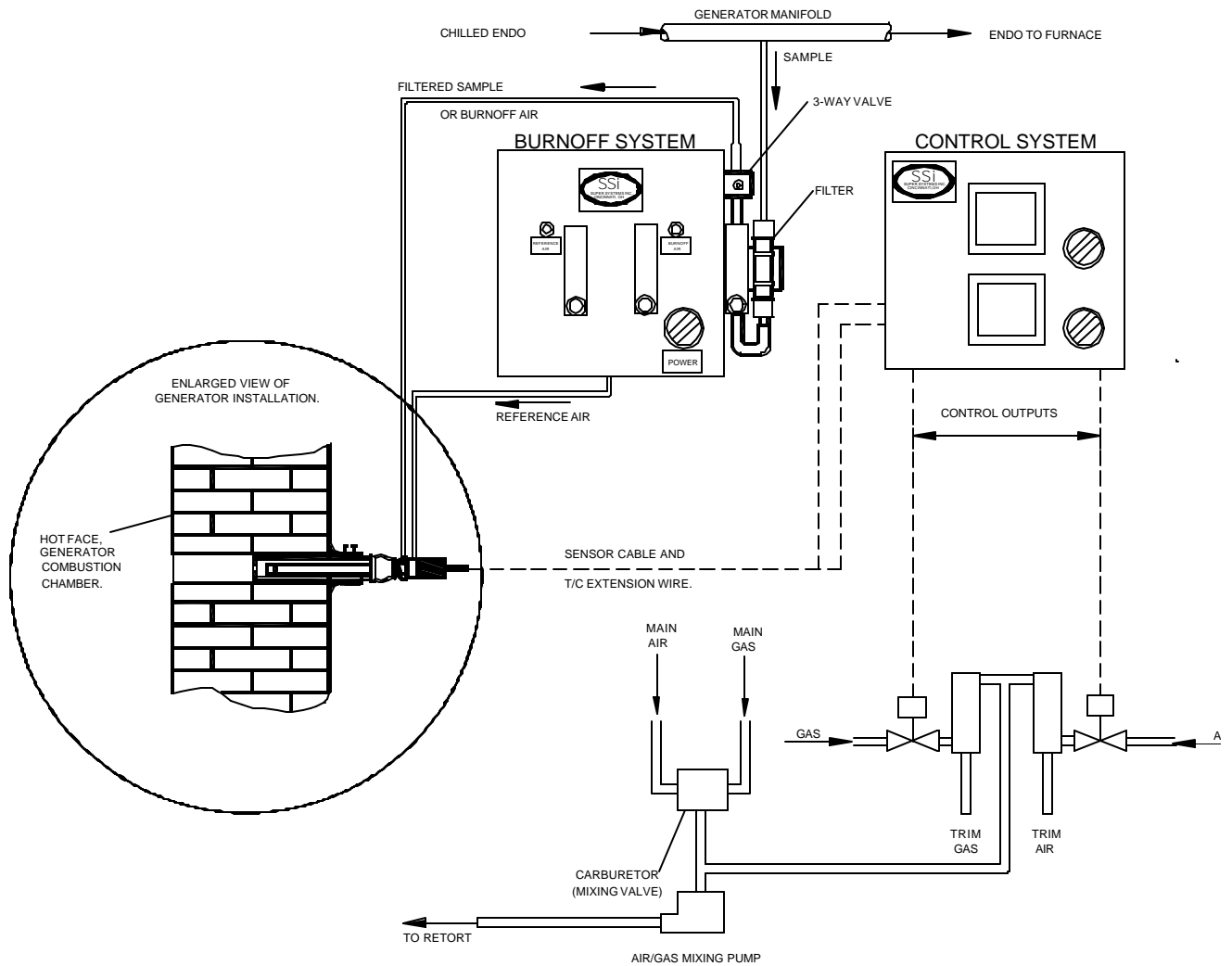
FIG.2 ENDOTHERMIC GENERATOR REHEAT WELL SAMPLING, CONDITIONING AND CONTROL SYSTEM
